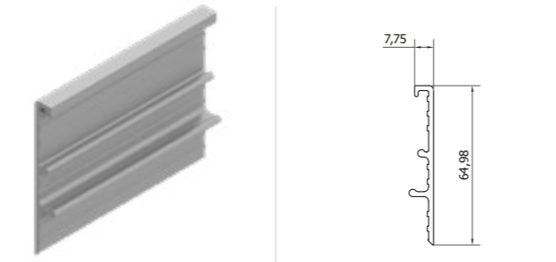
Deepfreeze Triple Glass Cover Profile Derin Dondurucu Isıcam Kapama Profili
