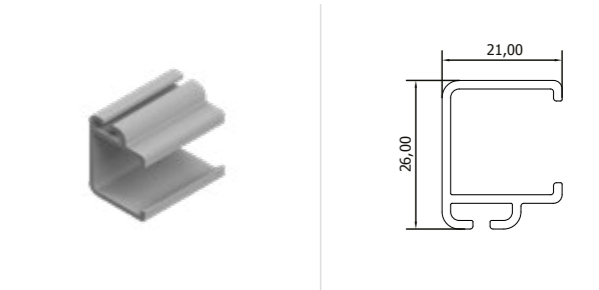
Glass Door Wing Profile Cam Kapı Kanat Profili
