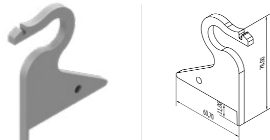
Solid Shelf Fixing Part Sac Raf Sabitleme Plastiği
