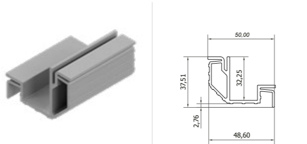
Deepfreeze Triple Glass Bottom Profile Derin Dondurucu Isıcam Alt Profili
