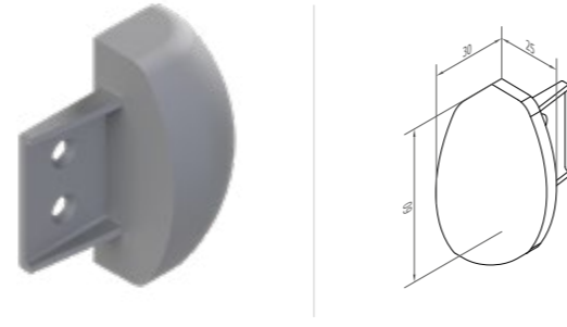
"D" Shaped Bumper Profile End Plastic "D" Tampon Profil Bitiş Plastiği
