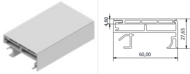
60' Case and Cover Profile 60'luk Kasa Kapak Profili
