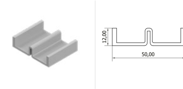
Sliding Rail Profile Sürgü Ray Profili
