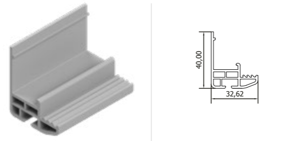
Glass Door Profile Cam Kapı Profili
