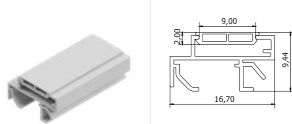
50' Case and Cover Profile 50'luk Kasa Kapak Profili
