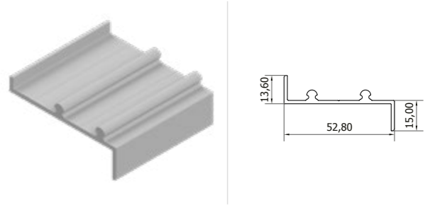
Sliding Rail Profile for Wheels Tekerli Sürgü Ray Profili
